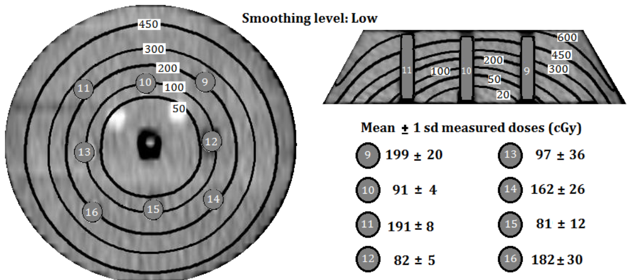
Figure 5 - Isodose distributions for the 2nd layer, using the low level of 3D Gaussian smoothing. All doses of the isodose lines are in cGy. The TLDs are shown in grey with their number code in white. At left, beam eye view taken at half height of the layer. At upper right, transversal view of the second layer.
