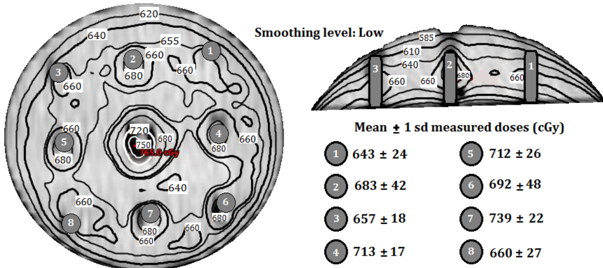
Figure 4 - Isodose distributions for the 1st layer, using the low level of 3D Gaussian smoothing. All doses of the isodose lines are in cGy. The TLDs are shown in grey with their number code in white. At left, beam eye view taken at half height of the layer. At upper right, transversal view of the first layer.
