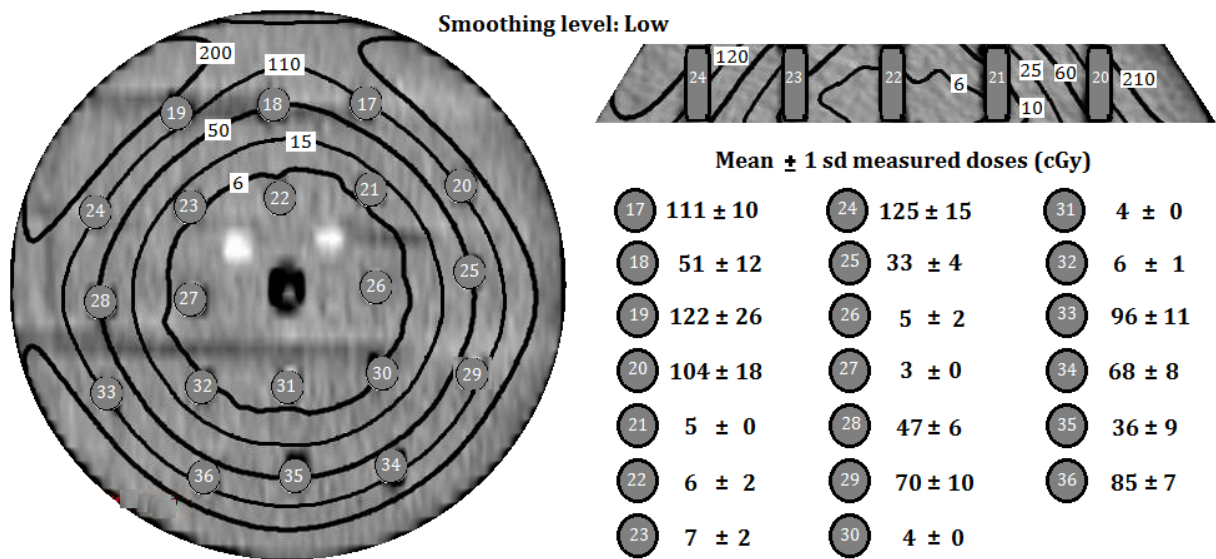
Figure 6 - Isodose distributions for the 3rd layer, using the low level of 3D Gaussian smoothing. All doses of the isodose lines are in cGy. The TLDs are shown in grey with their number code in white. At left, beam eye view taken at half height of the layer. At upper right, transversal view of the third layer.
